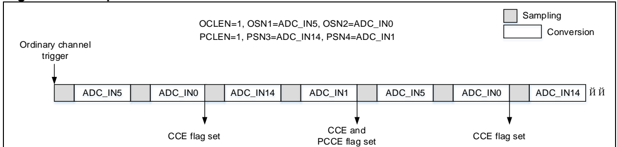
Figure 18-6 Repetition mode
