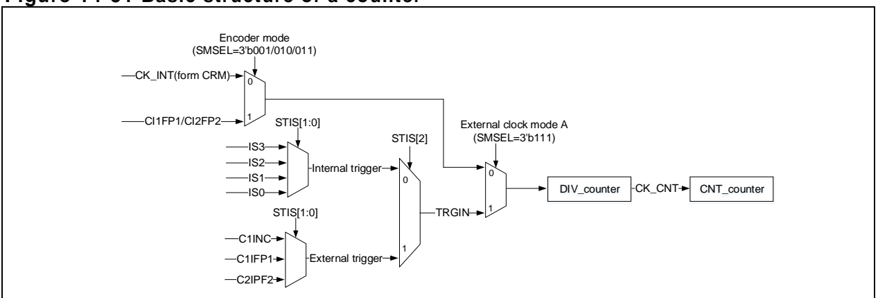
Figure 14-51 Basic structure of a counter
