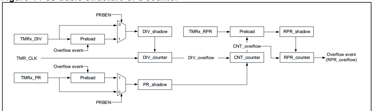
Figure 14-99 Basic structure of a counter
