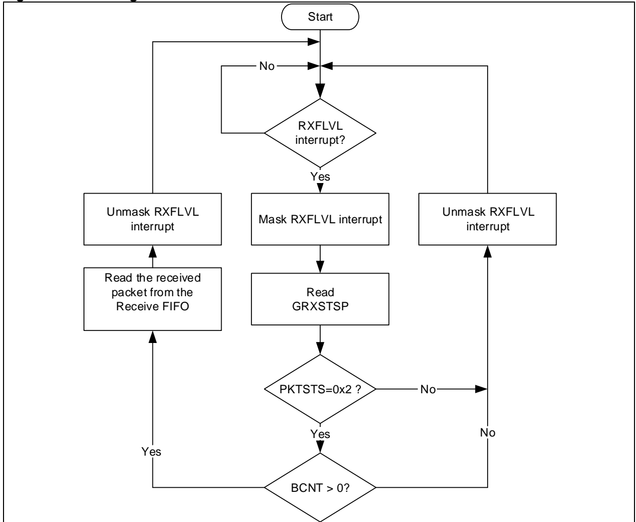
Figure 20-4 Reading the receive FIFO
