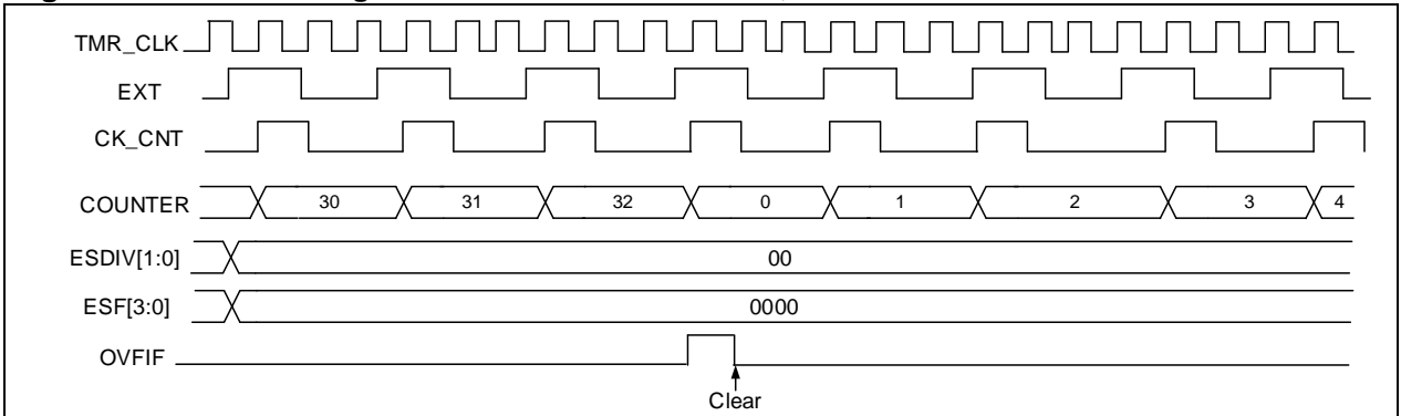
Figure 14-97 Counting in external clock mode B, PR=0x32, DIV=0x0
