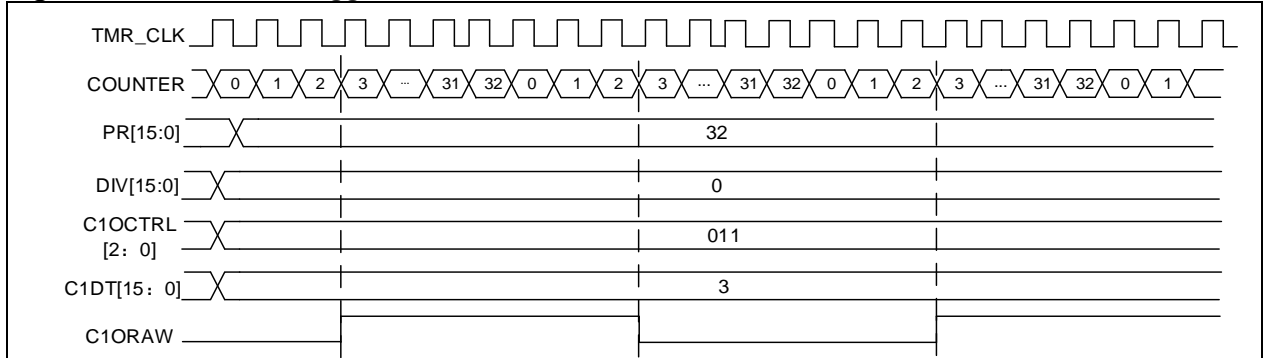
Figure 14-86 Upcounting mode and PWM mode A
