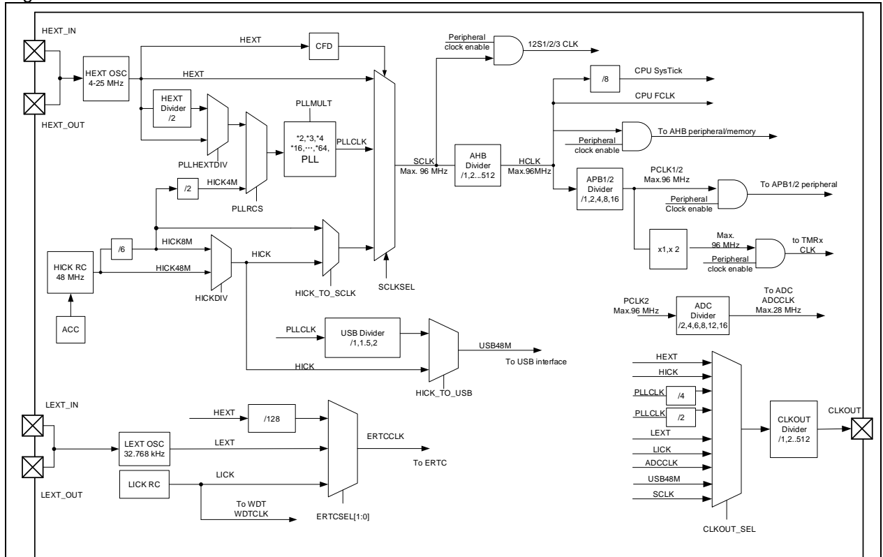
Figure 4-1 AT32F425 clock tree
