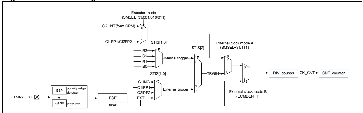
Figure 14-92 Counting clock
