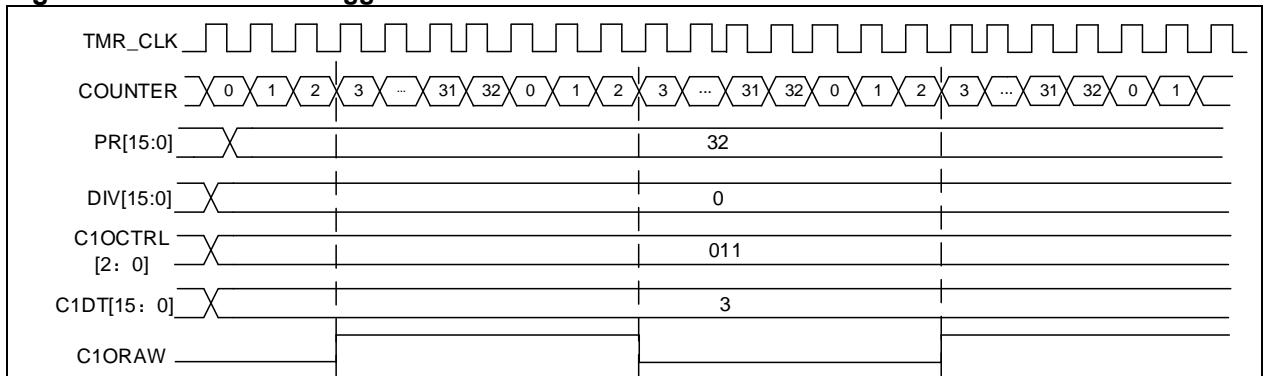
Figure 14-113 C1ORAW toggles when counter value matches the C1DT value
