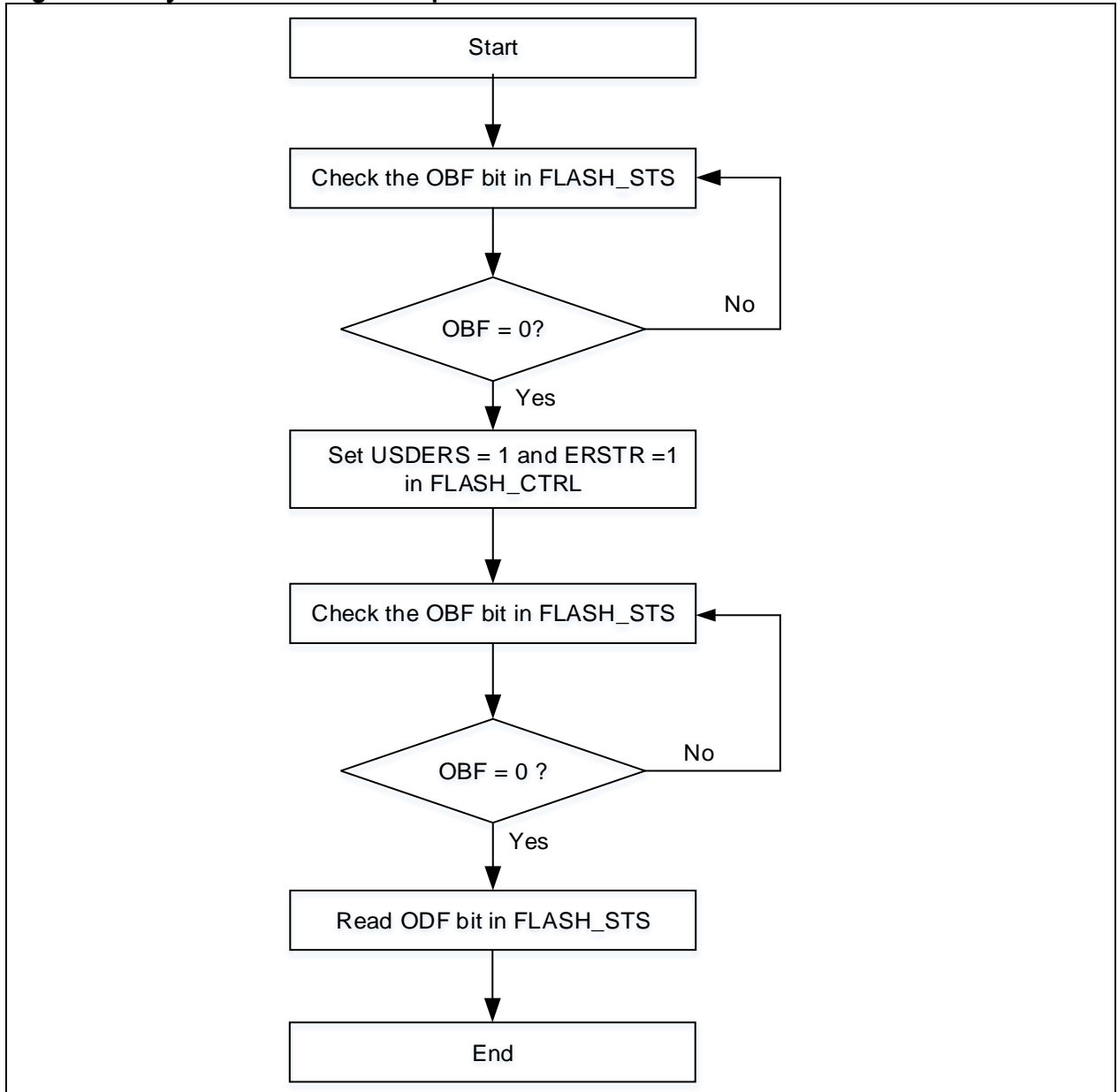
Figure 5-4 System data area erase process
