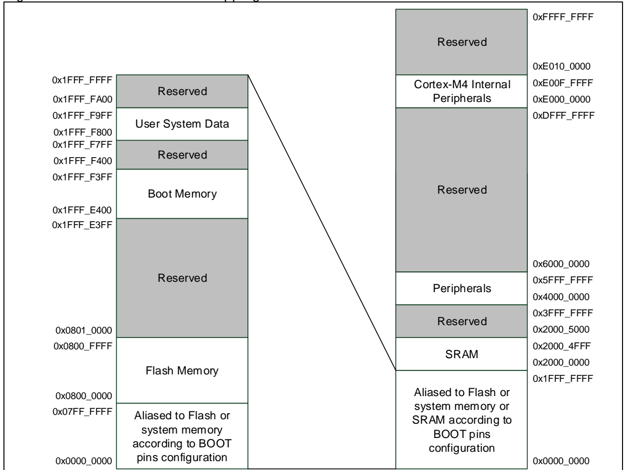
Figure 2-1 AT32F425 address mapping
