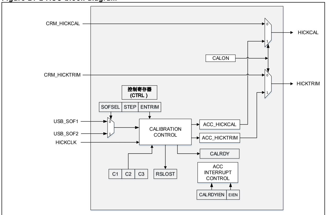
Figure 21-2 ACC block diagram
