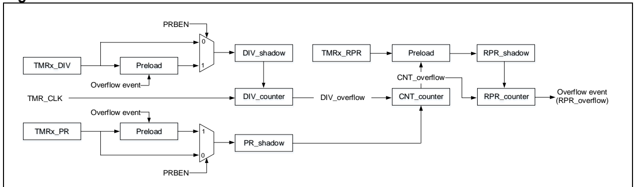
Figure 14-56 Basic structure of a counter
