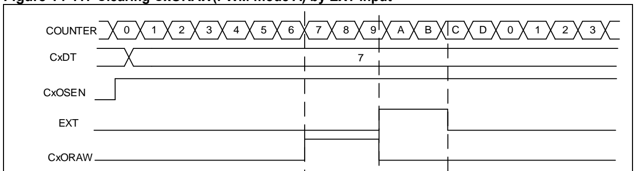
Figure 14-117 Clearing CxORAW(PWM mode A) by EXT input
