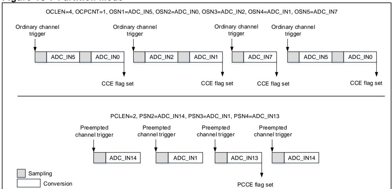
Figure 18-7 Partition mode
