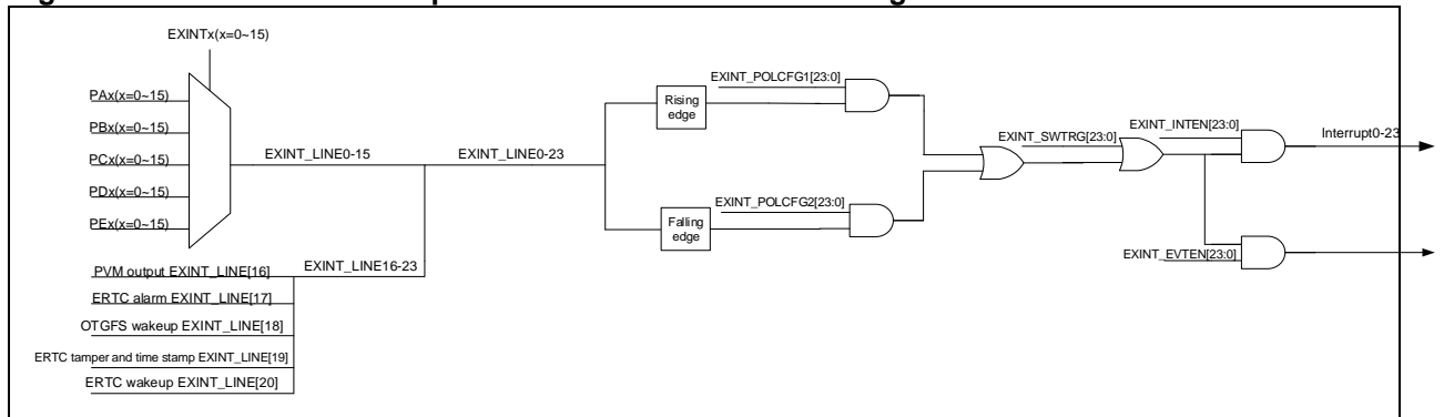
Figure 8-1 External interrupt/Event controller block diagram
