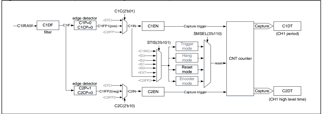
Figure 14-110 PWM input mode
