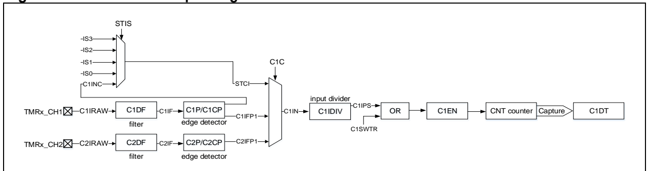
Figure 14-61 Channel 1 input stage
