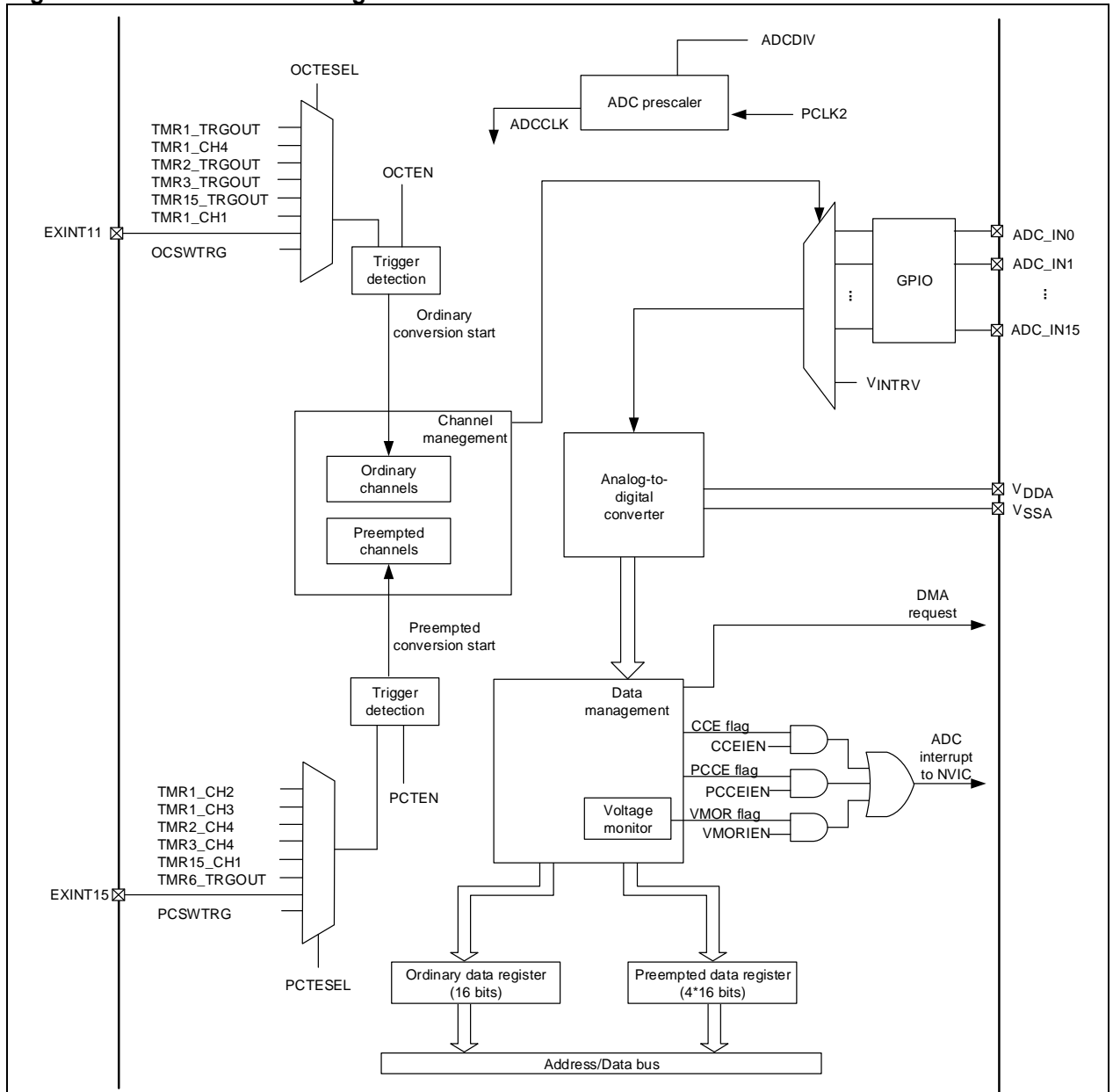
Figure 18-1 ADC1 block diagram
