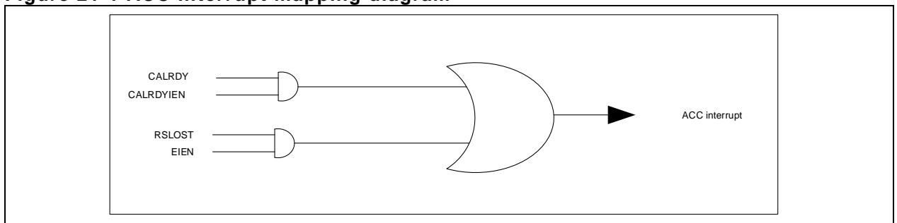
Figure 21-1 ACC interrupt mapping diagram
