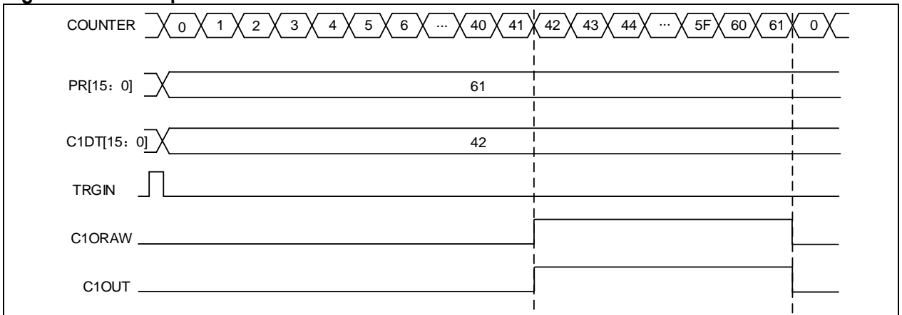
Figure 14-49 One-pulse mode
