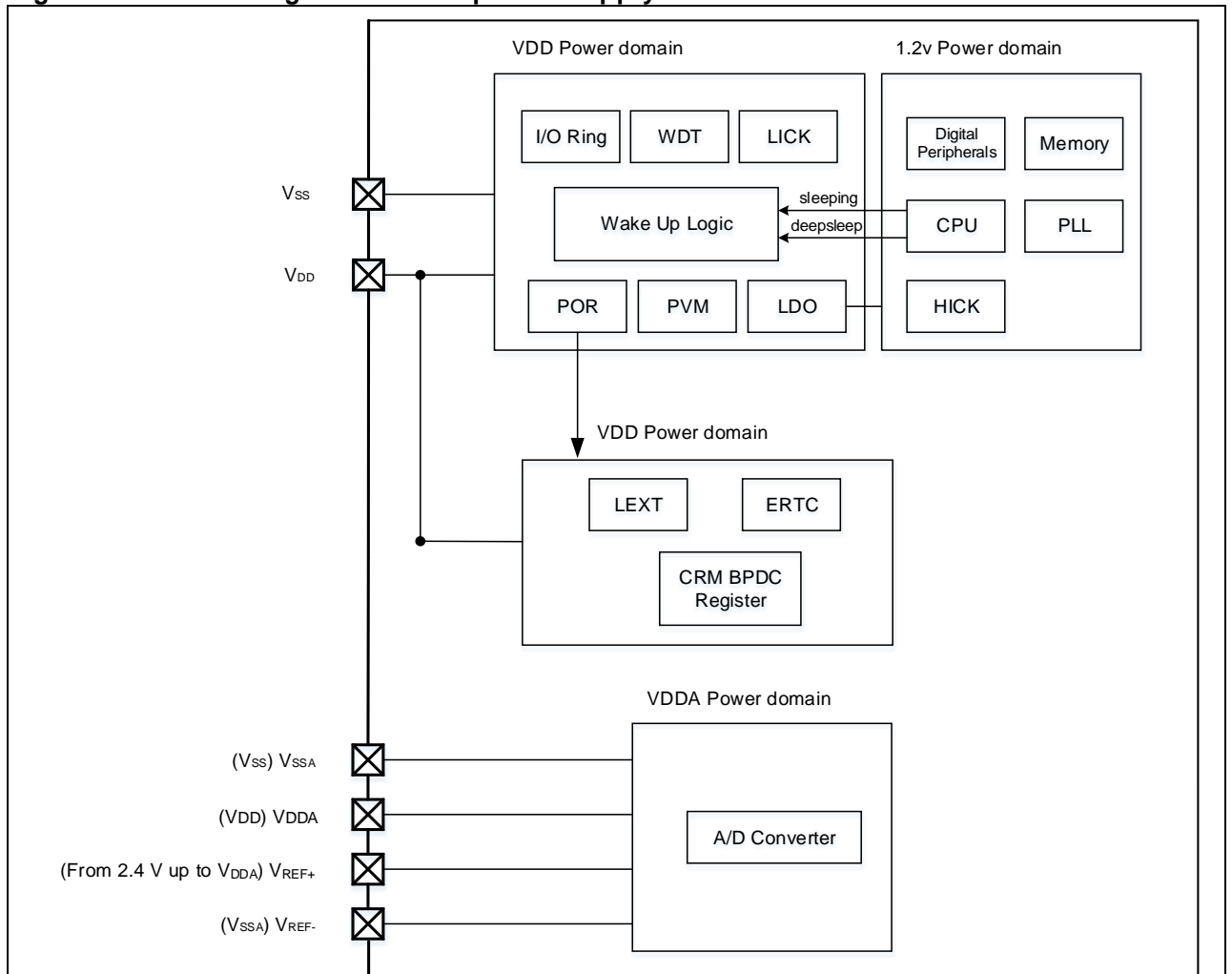
Figure 3-1 Block diagram of each power supply
