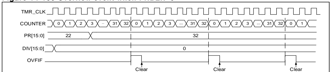
Figure 14-100 Overflow event when PRBEN=0
