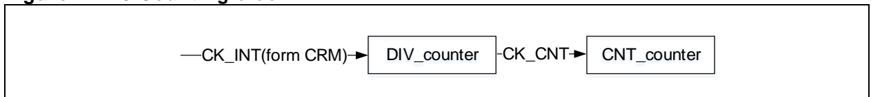
Figure 14-76 Counting clock
