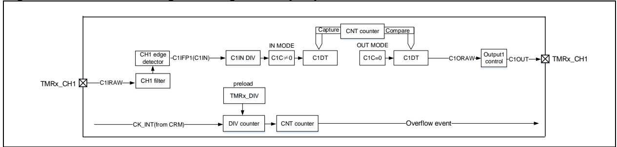
Figure 14-38 Block diagram of general-purpose TMR13/14
