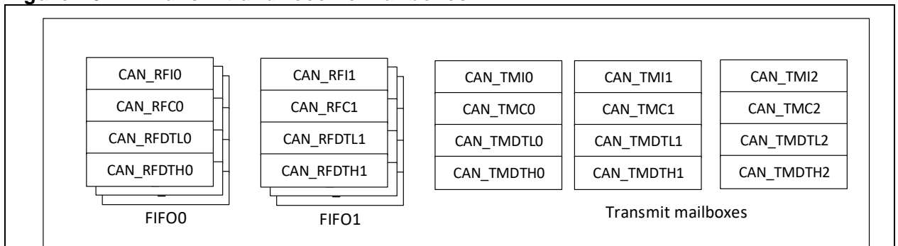
Figure 19-14 Transmit and receive mailboxes
