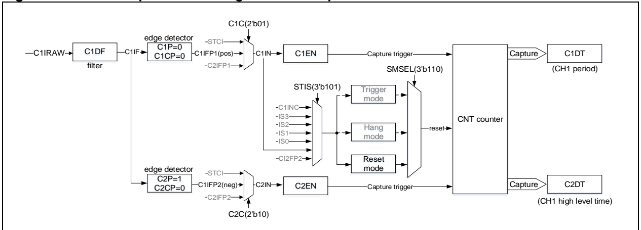
Figure 14-63 PWM input mode
