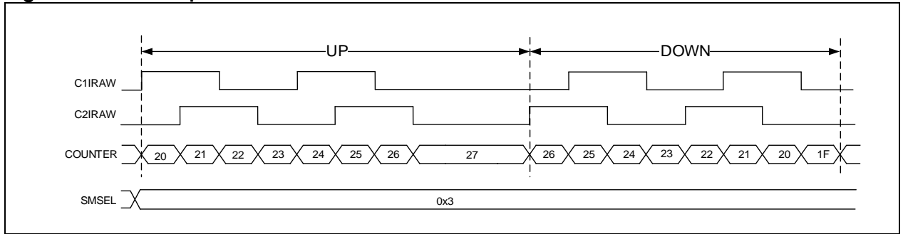
Figure 14-106 Example of encoder interface mode C
