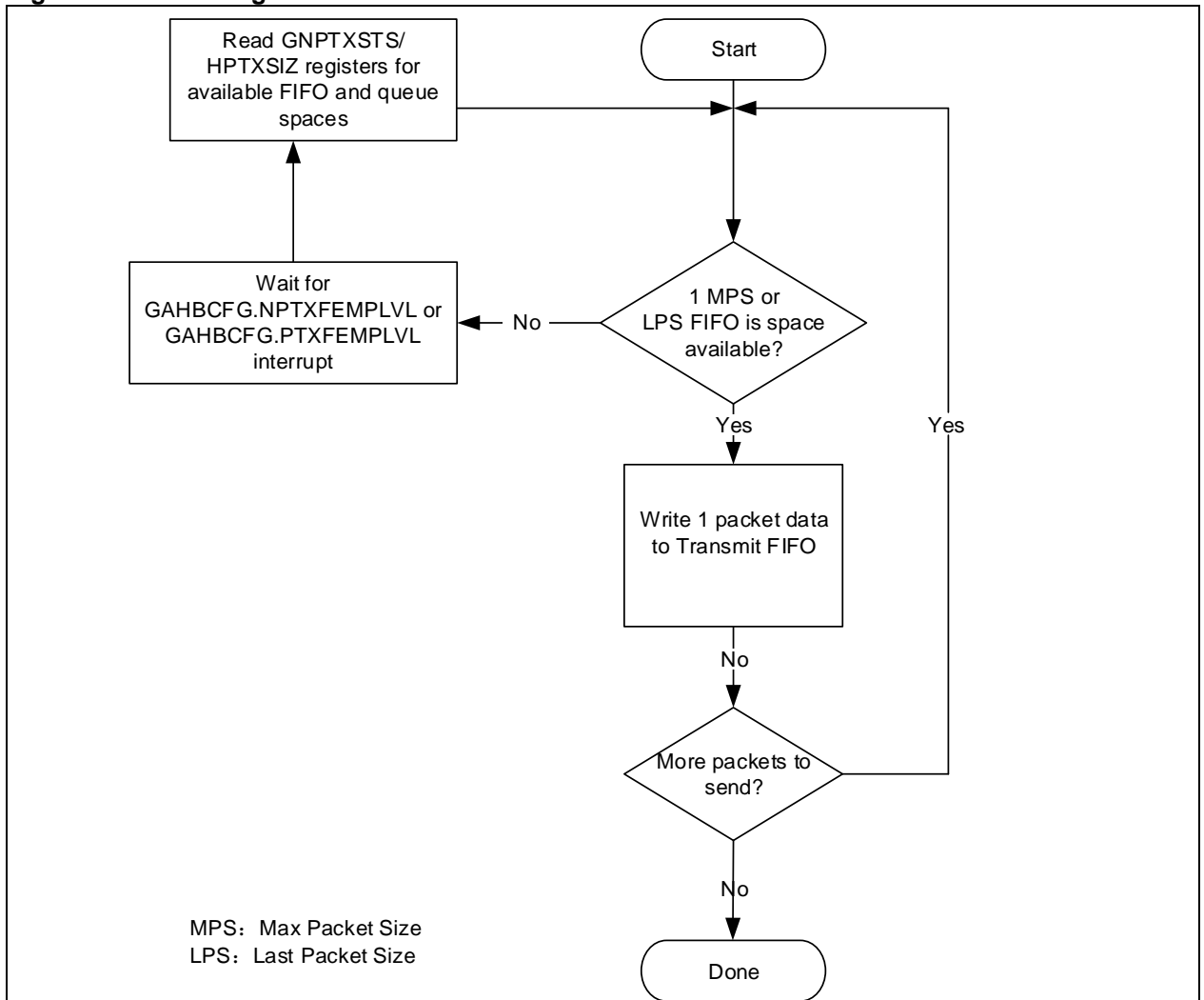
Figure 20-3 Writing the transmit FIFO
