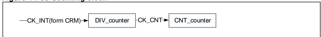
Figure 14-39 Counting clock
