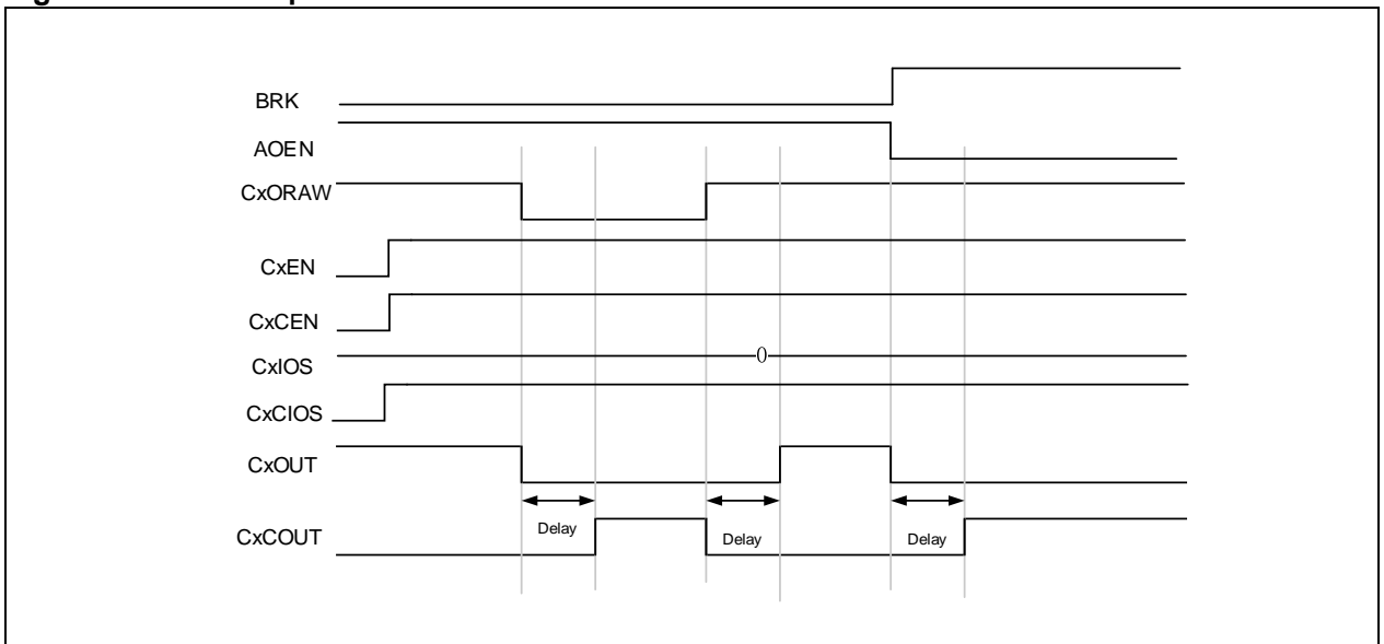
Figure 14-120 Example of TMR break function
