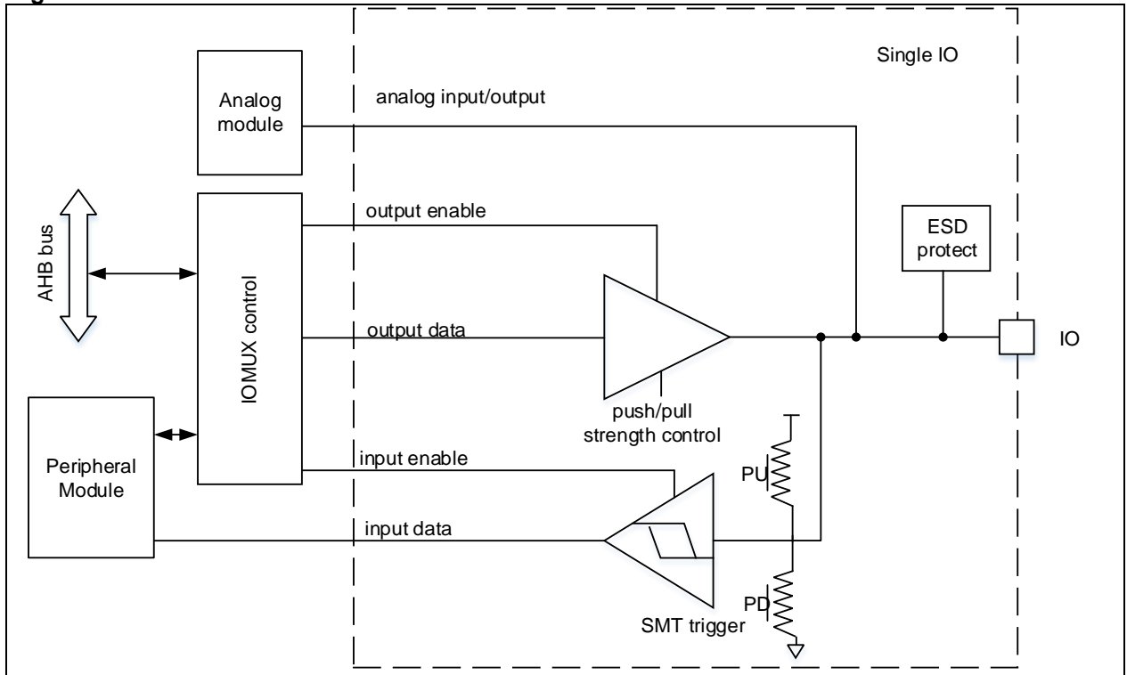
Figure 6-2 IOMUX structure
