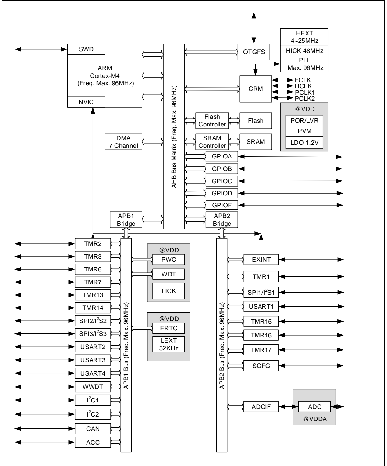
Figure 1-1 AT32F425 Series microcontrollers system architecture
