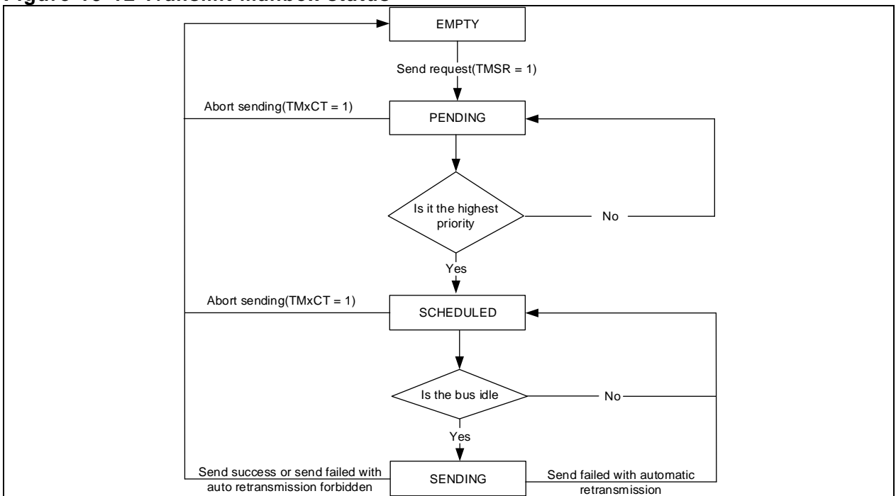
Figure 19-12 Transmit mailbox status
