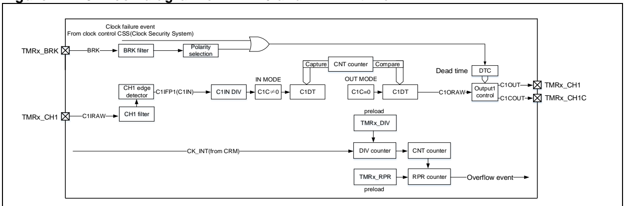
Figure 14-75 Block diagram of TMR16 and TMR17 timer
