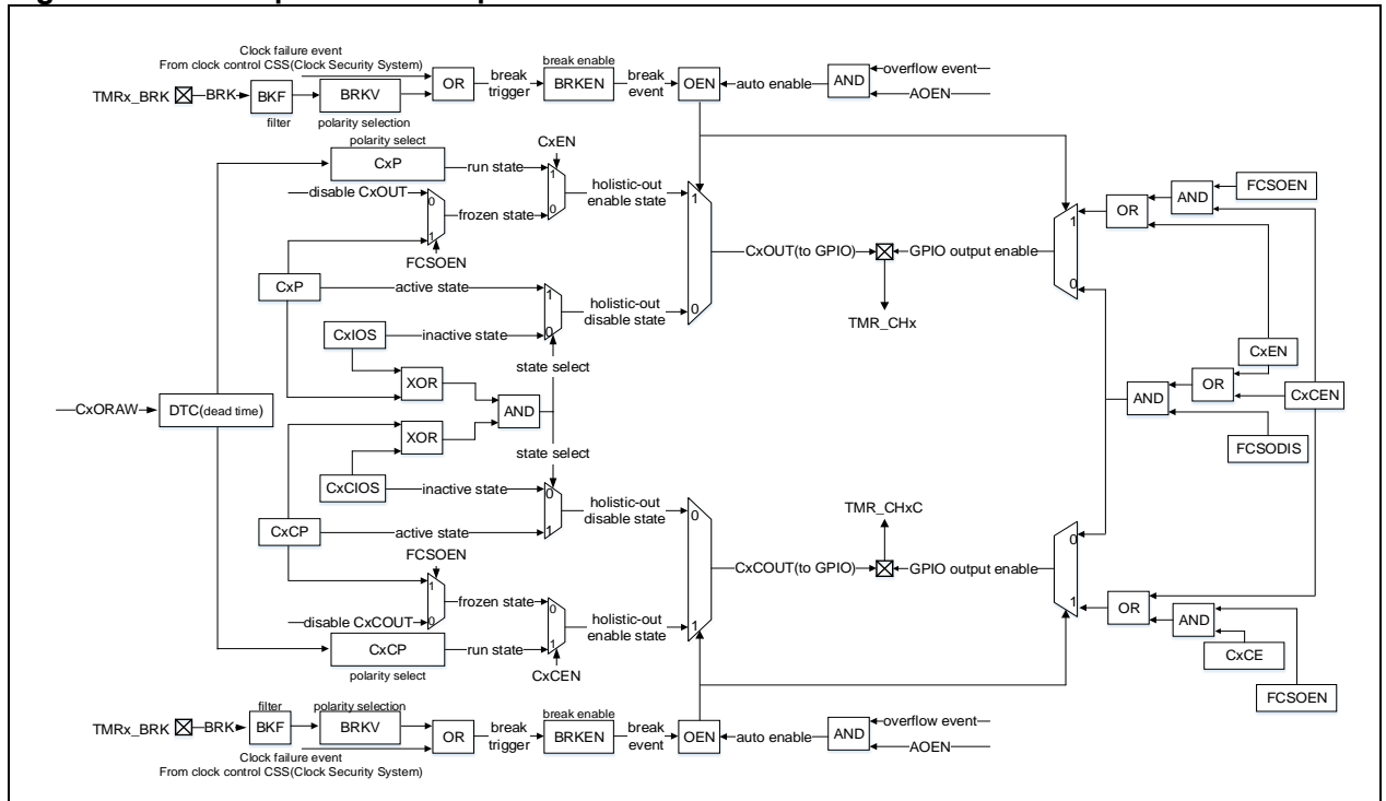
Figure 14-90 Example of TMR break function
