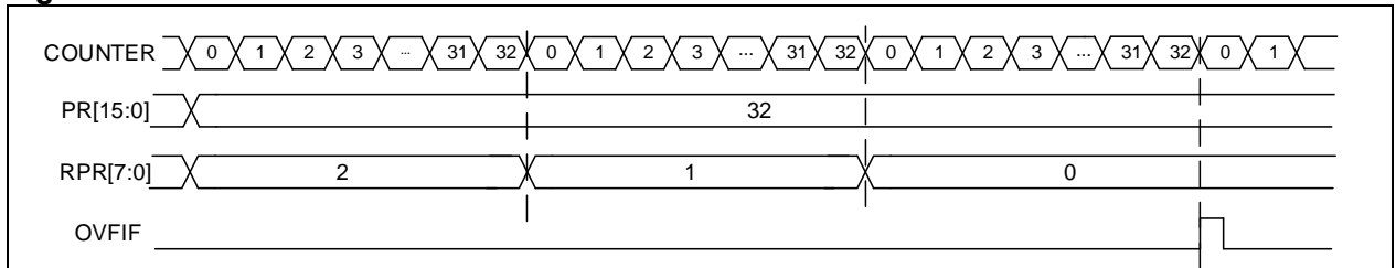
Figure 14-81 OVFIFF when RPR=2
