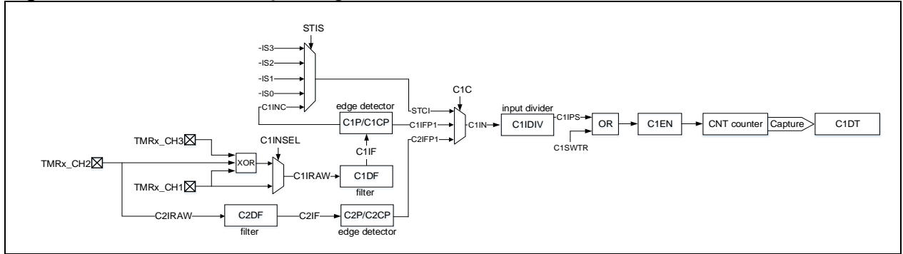
Figure 14-108 Channel 1 input stage
