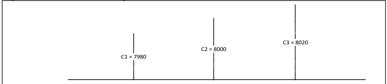
Figure 21-3 Cross-return algorithm
