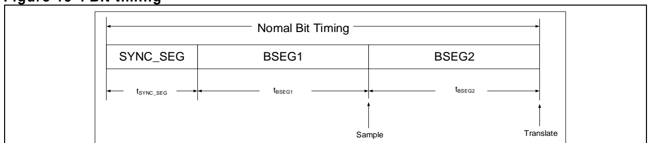
Figure 19-1 Bit timing
