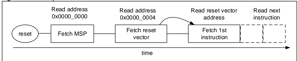
Figure 1-5 Reset process
