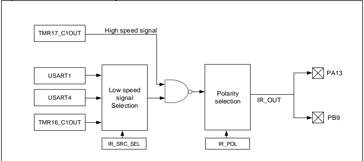
Figure 22-1 IRTMR block diagram
