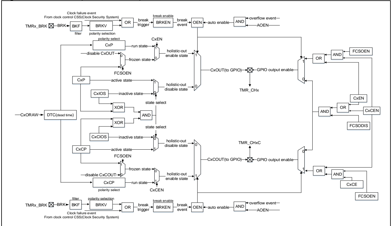
Figure 14-120 Example of TMR break function
