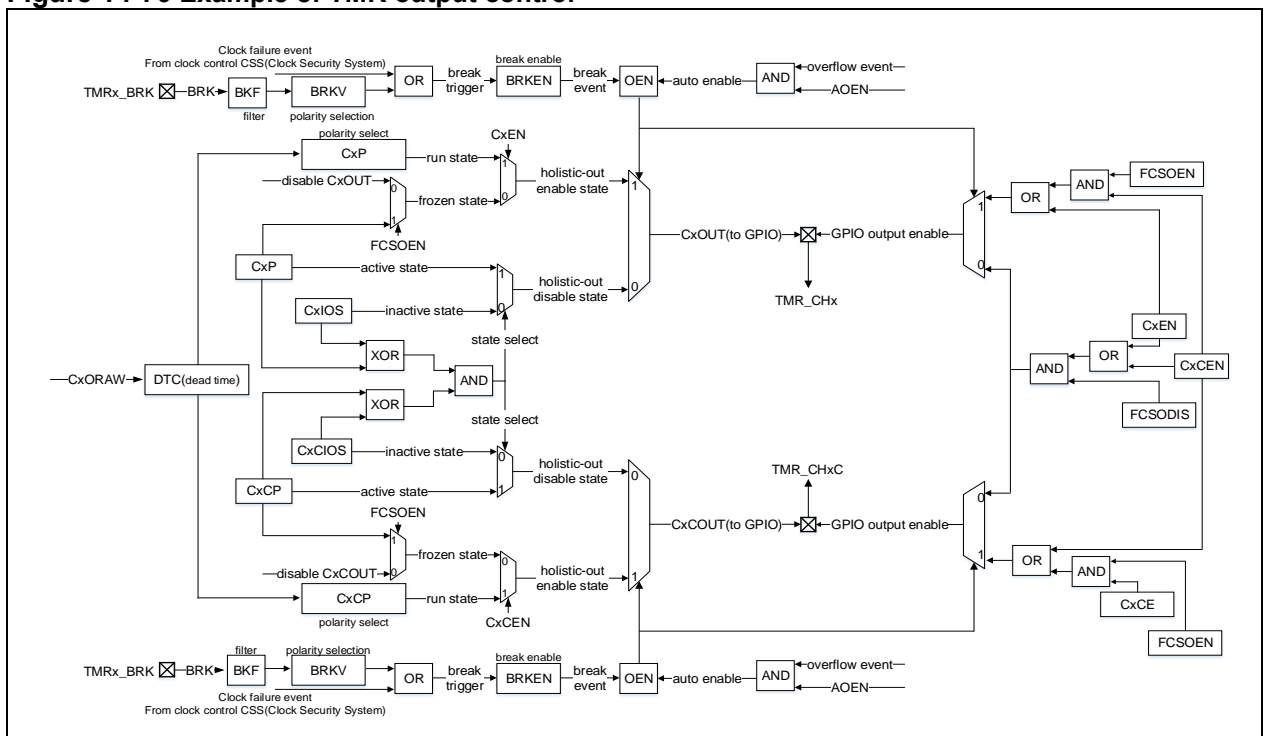
Figure 14-70 Example of TMR output control
