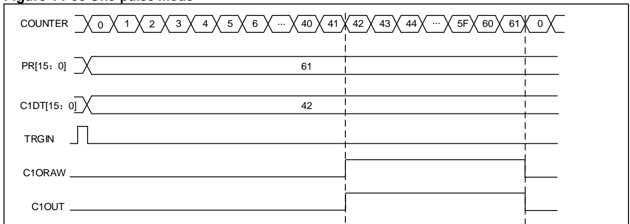
Figure 14-68 One-pulse mode
