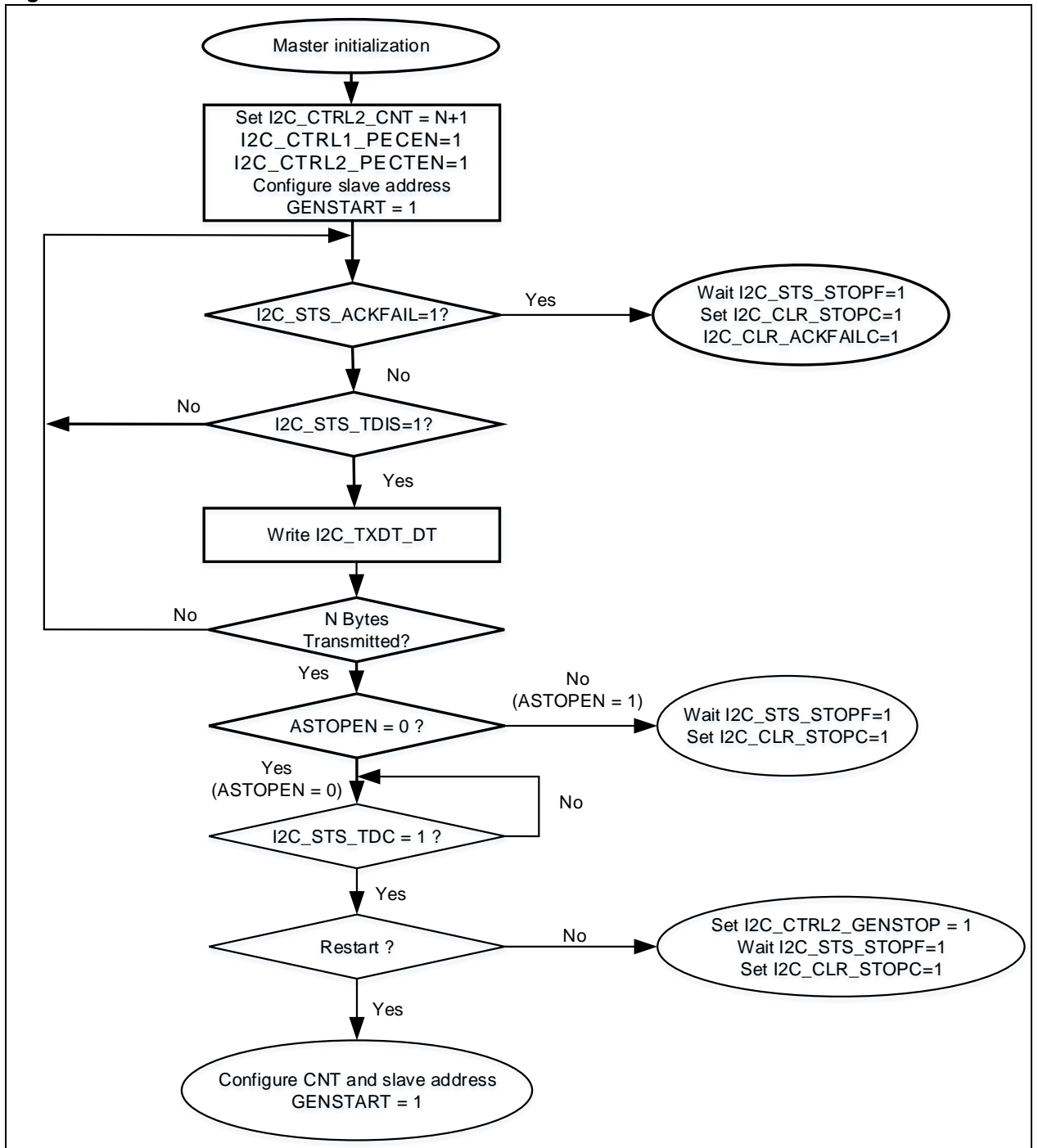
SMBus master transmission flow Figure 11-14 SMBus master transmission flow
