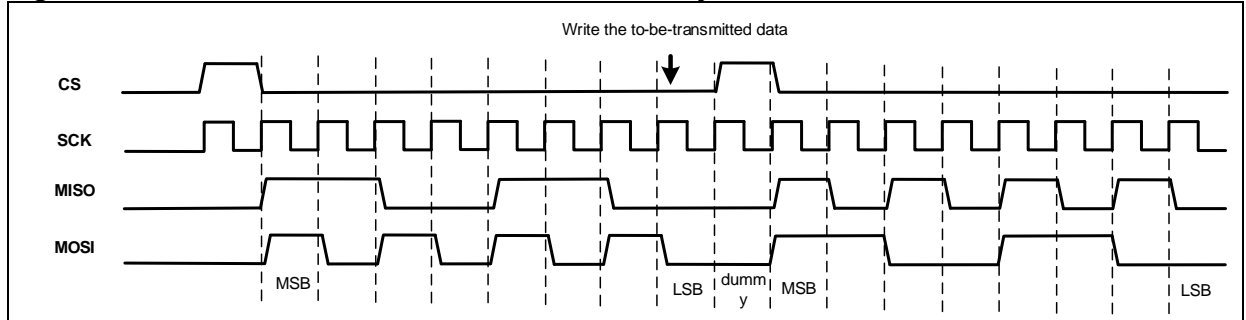
Figure 13-13 TI mode continous transfer with dummy CLK
