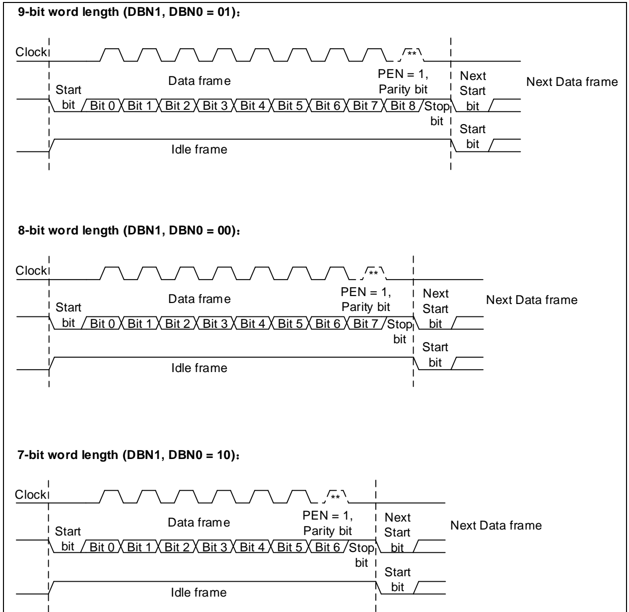
Figure 12-8 Word length
