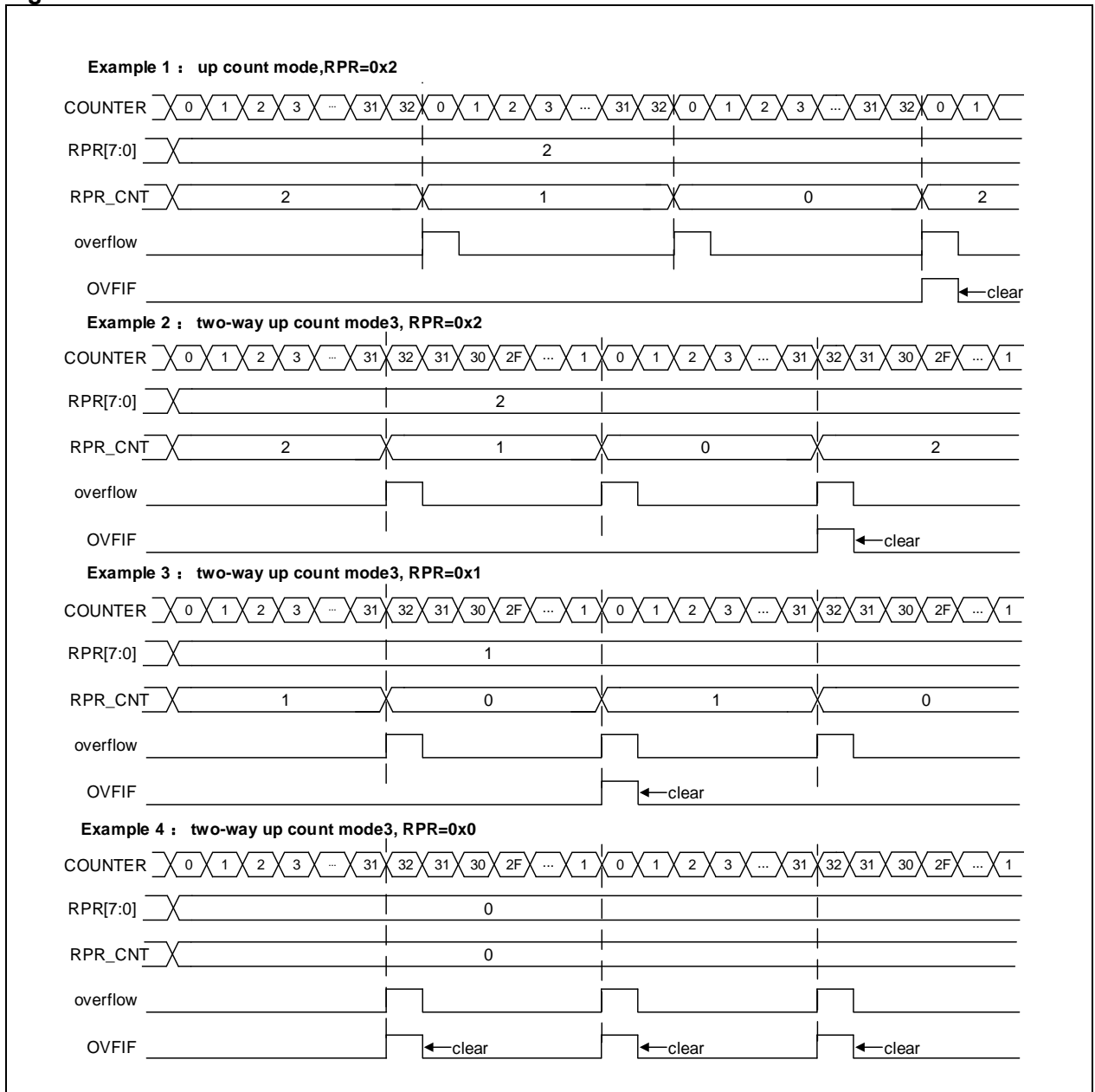
Figure 14-104 OVIF when RPR=2
