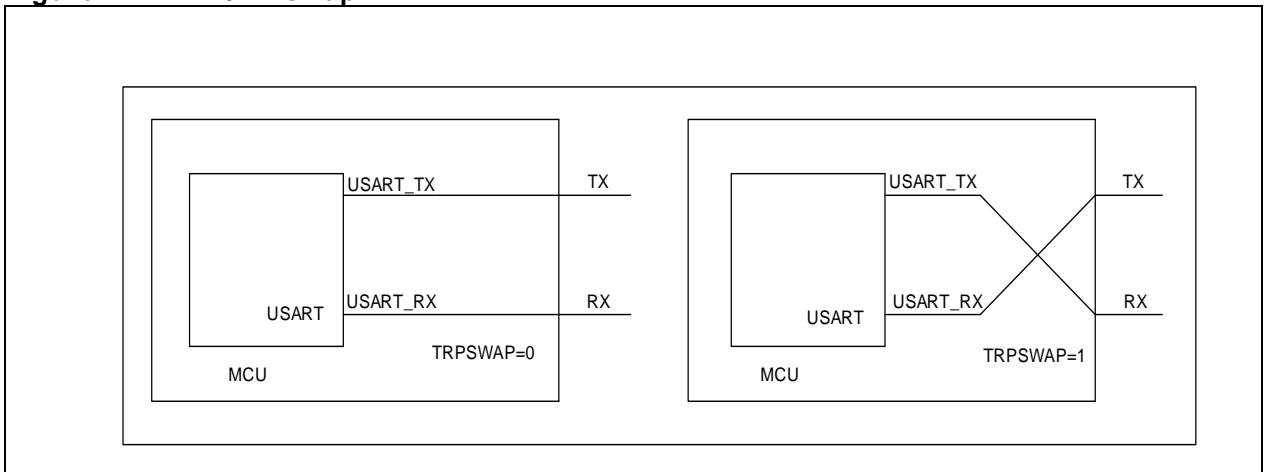
Figure 12-12 Tx/Rx swap
