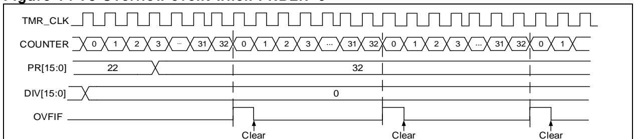
Figure 14-79 Overflow event when PRBEN=0
