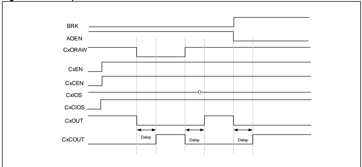
Figure 14-90 Example of TMR break function
