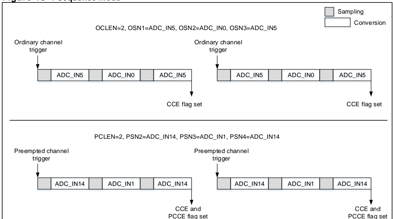
Figure 18-4 Sequence mode
