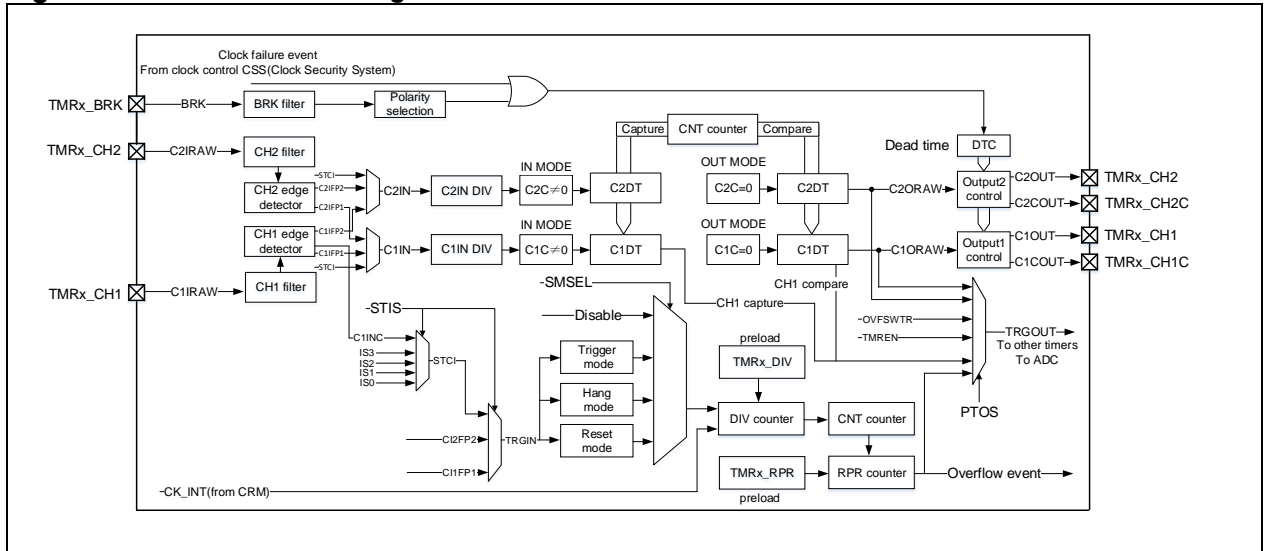
Figure 14-50 TMR15 block diagram
