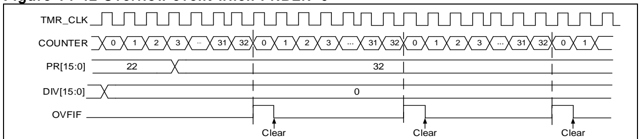
Figure 14-43 Overflow event when PRBEN=1
