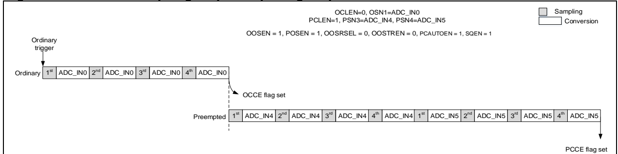
Figure 18-10 Oversampling of preempted group of channels
