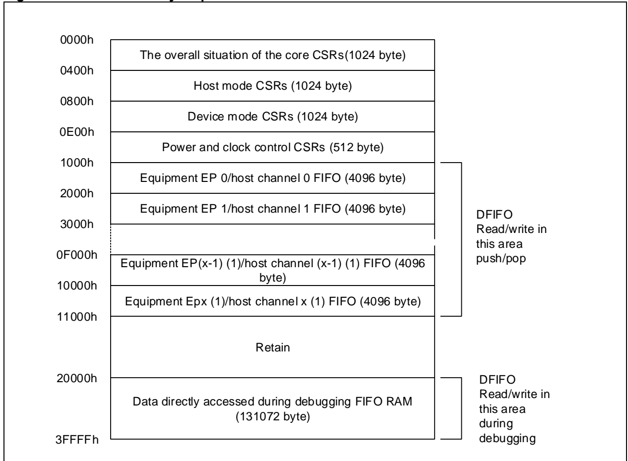
Figure 20-13 CSR memory map
