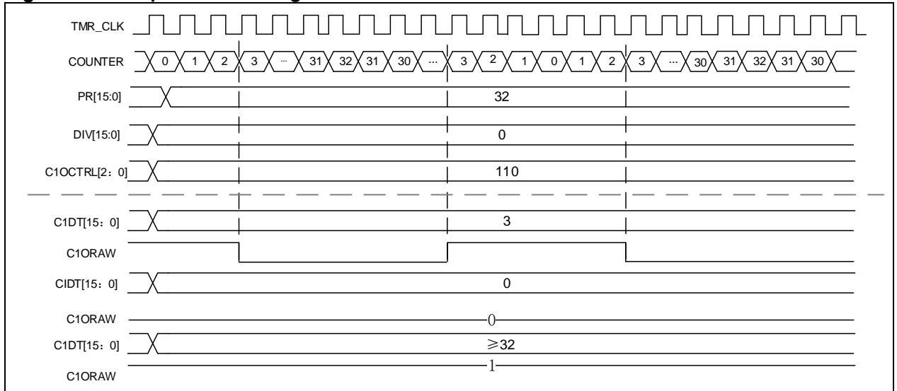
Figure 14-115 Up/down counting mode and PWM mode
