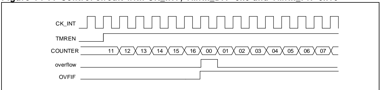
Figure 14-77 Control circuit with CK_INT, TMRx_DIV=0x0 and TMRx_PR=0x16
