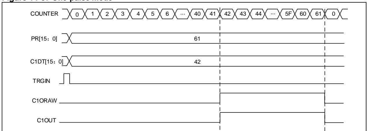
Figure 14-87 One-pulse mode
