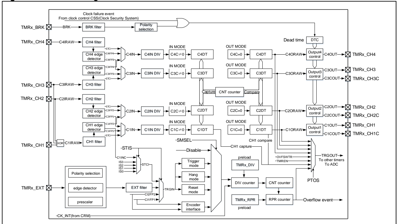
Figure 14-91 Block diagram of advanced-control timer
