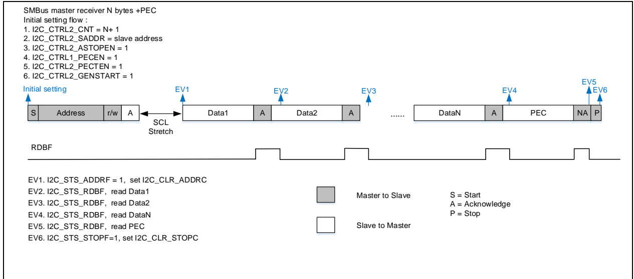
Figure 11-17 SMBus master receive timing
