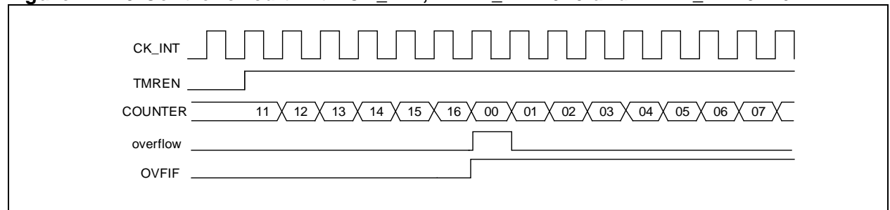
Figure 14-40 Control circuit with CK_INT, TMRx_DIV=0x0 and TMRx_PR=0x16
