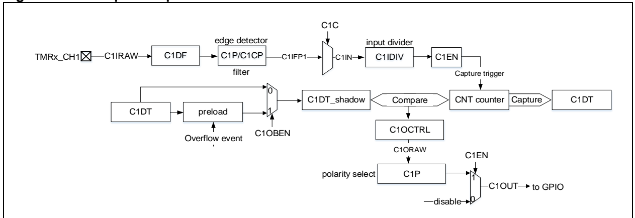
Figure 14-45 Channel 1 input stage
