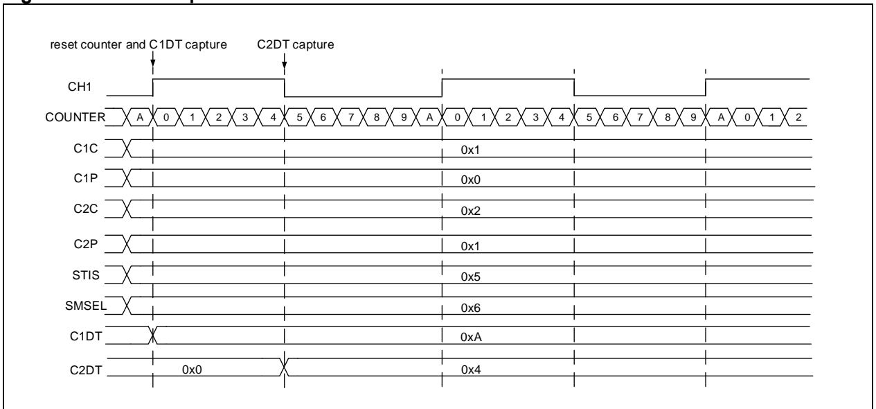
Figure 14-63 PWM input mode
