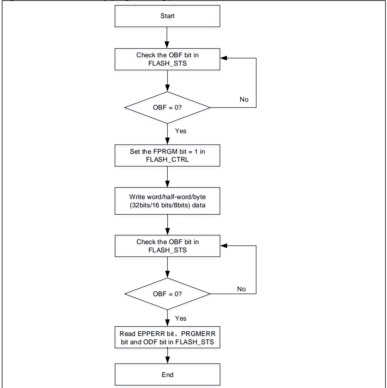
Figure 5-3 Flash memory programming process
