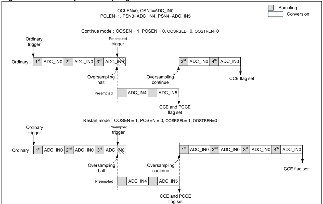
Figure 18-8 Ordinary oversampling restart mode selection
