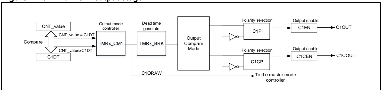
Figure 14-64 Channel 1 output stage
