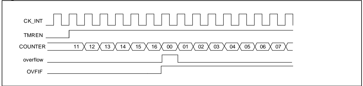
Figure 14-93 Control circuit with CK_INT, TMRx_DIV=0x0 and TMRx_PR=0x16
