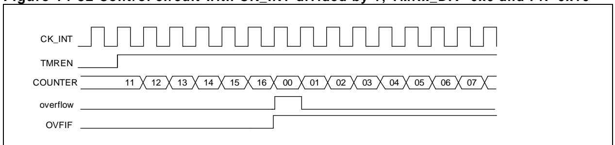
Figure 14-52 Control circuit with CK_INT divided by 1, TMRx_DIV=0x0 and PR=0x16
