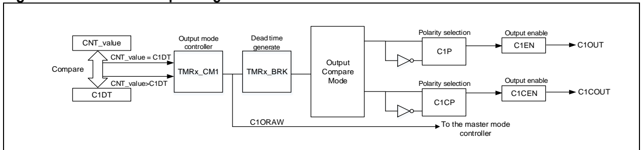
Figure 14-84 Channel output stage
