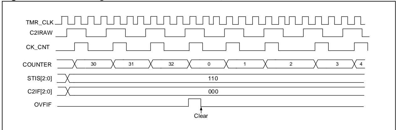
Figure 14-54 Counting in external clock mode A, PR=0x32, DIV=0x0
