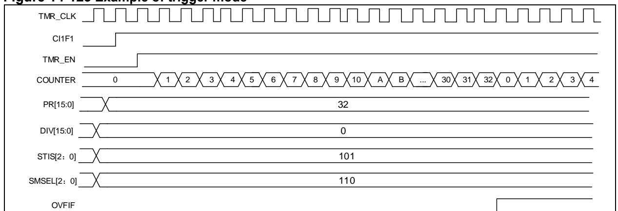
Figure 14-123 Example of trigger mode
