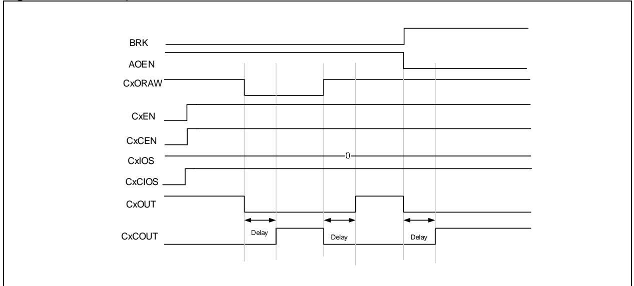
Figure 14-71 Example of TMR break function
