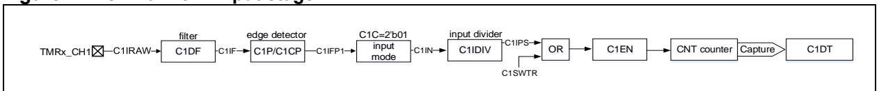
Figure 14-45 Channel 1 input stage
