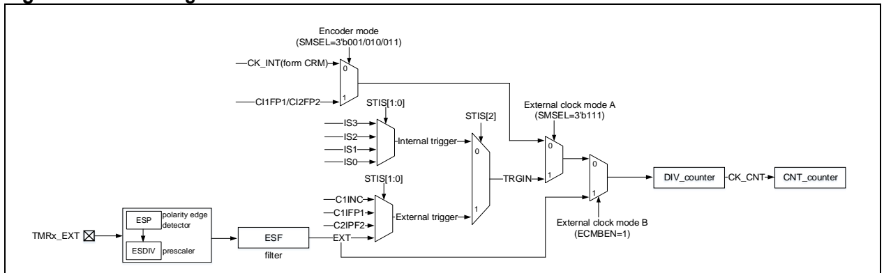
Figure 14-8 Counting clock
