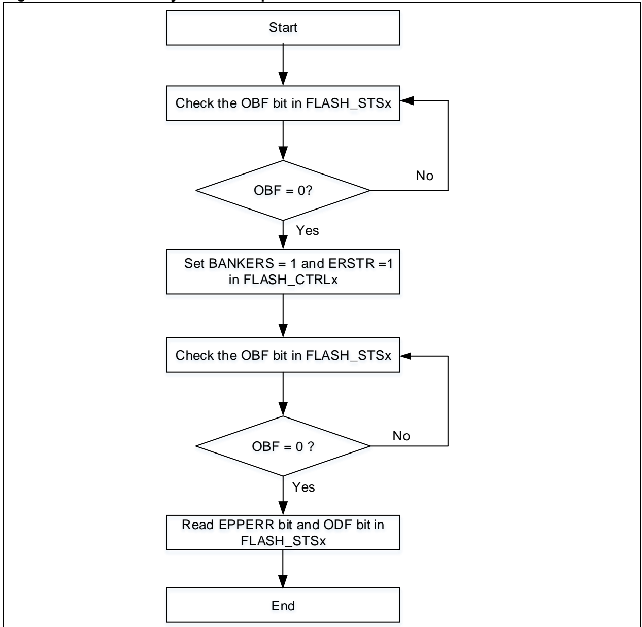
Figure 5-2 Flash memory bank erase process
